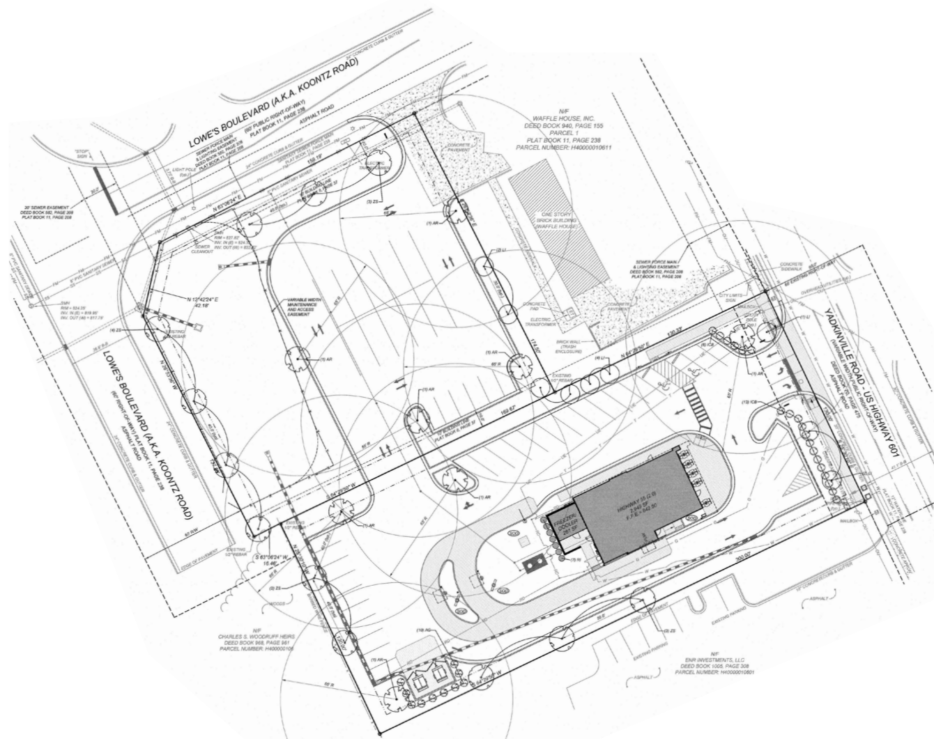
SITE PLAN
