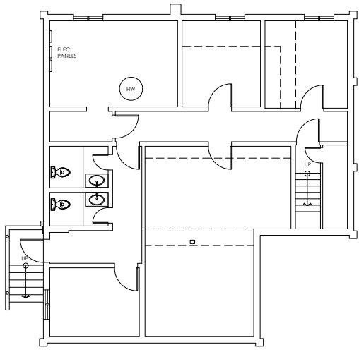
Existing Basement Floor Plan
