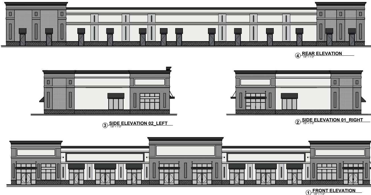
UPDATED PAINT RENDERINGS
